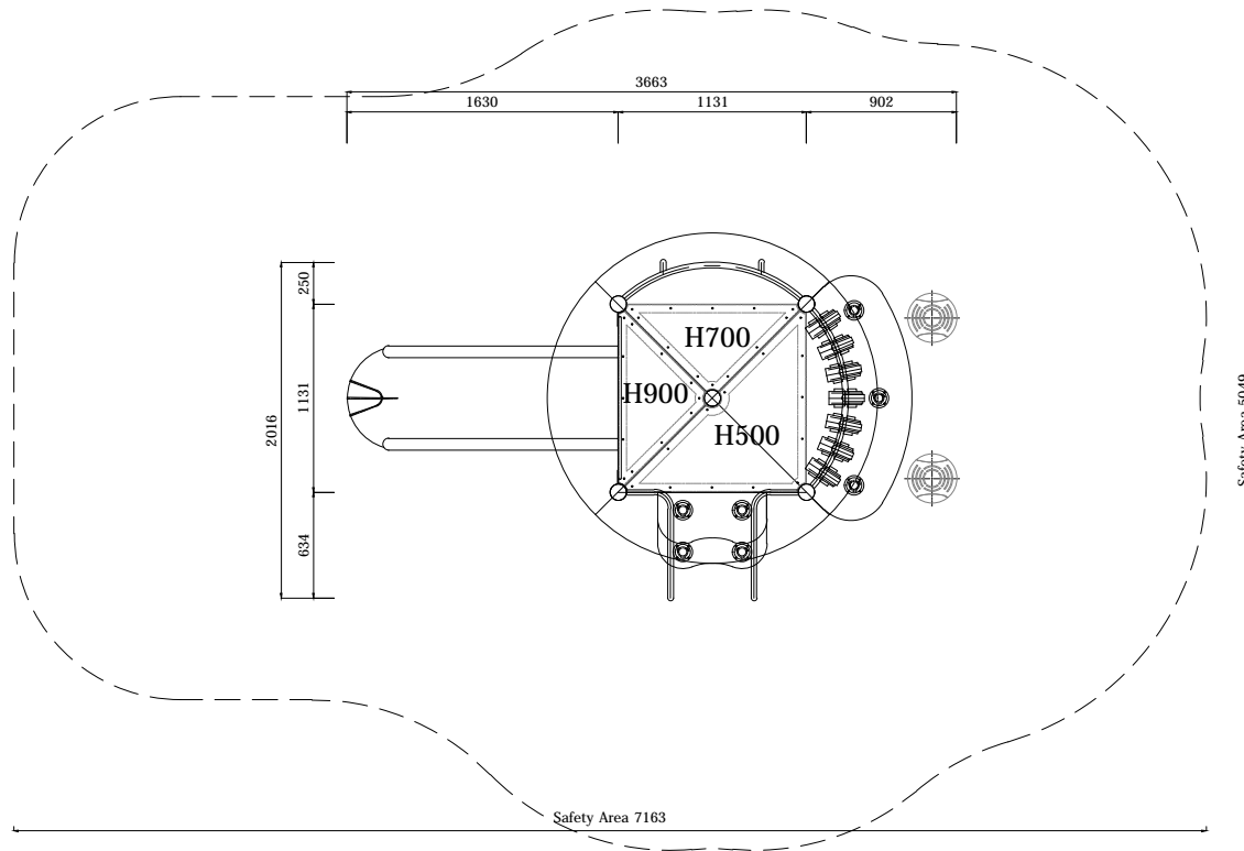
PLAN LAYOUT
