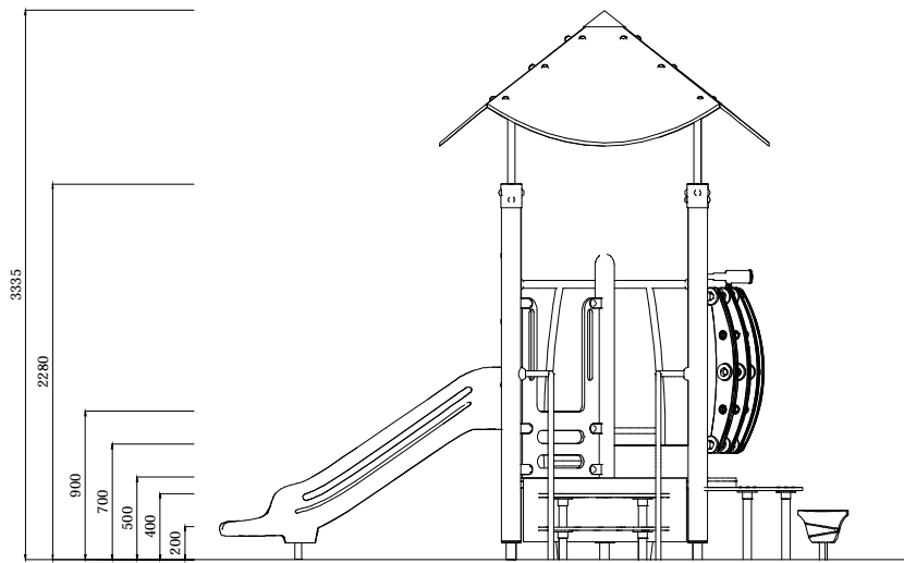
ELEVATION - FRONT
