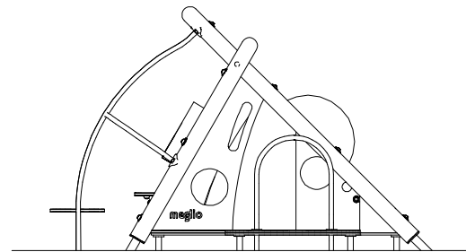
FOOTING LAYOUT
