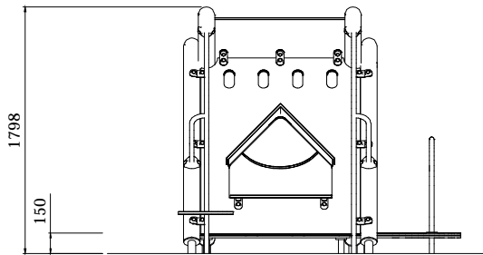
PLAN LAYOUT
