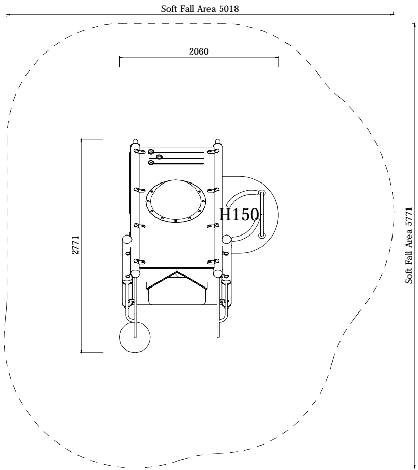
PLAN LAYOUT
