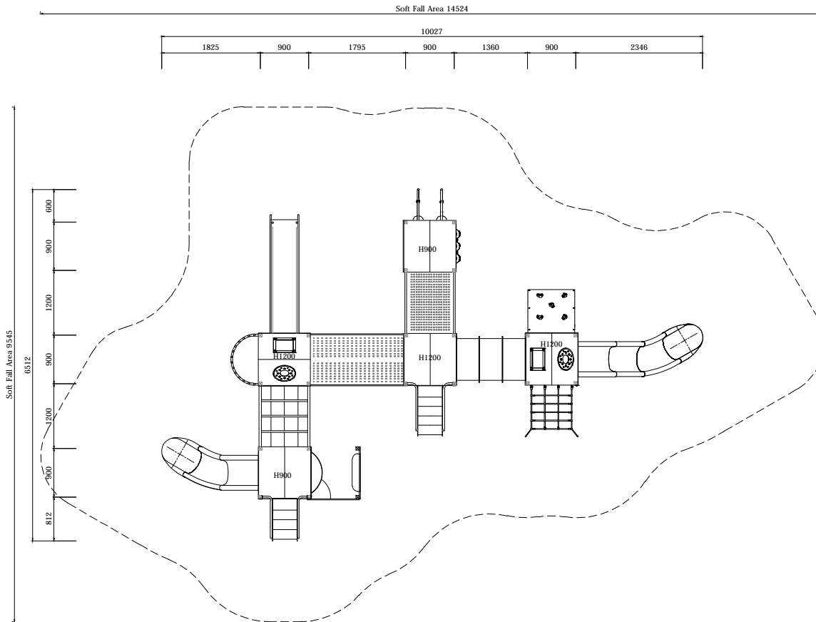
PLAN LAYOUT
