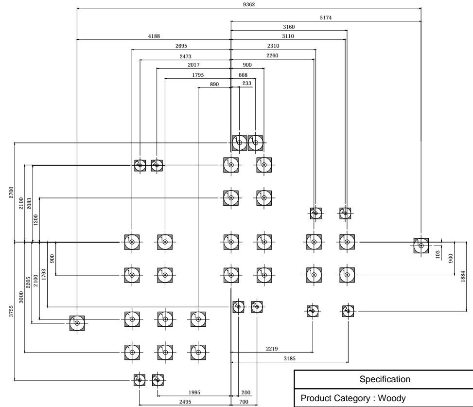
FOOTING LAYOUT
