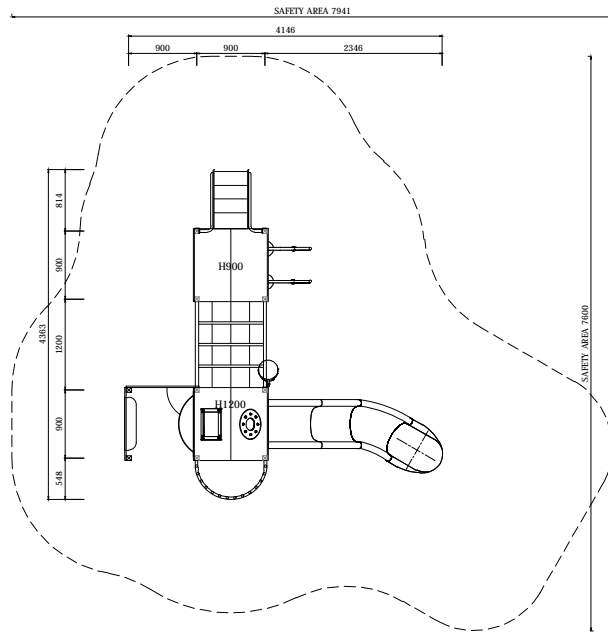
PLAN LAYOUT
