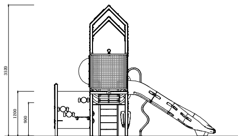
ELEVATION - FRONT
