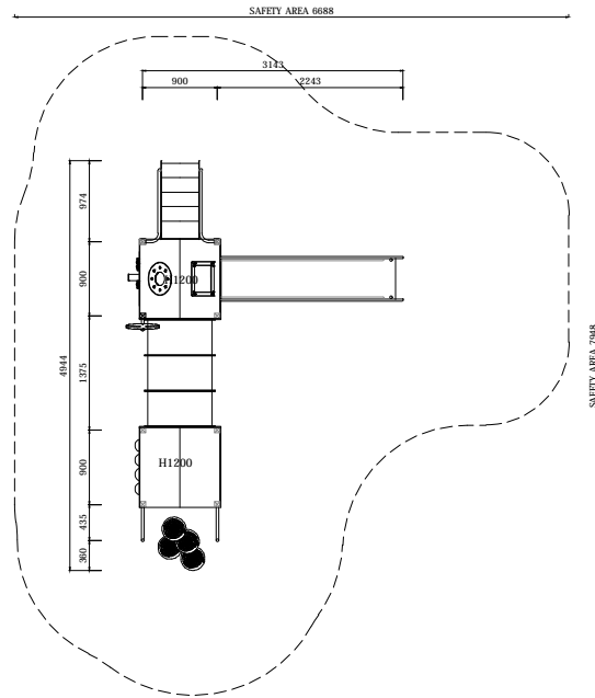
PLAN LAYOUT
