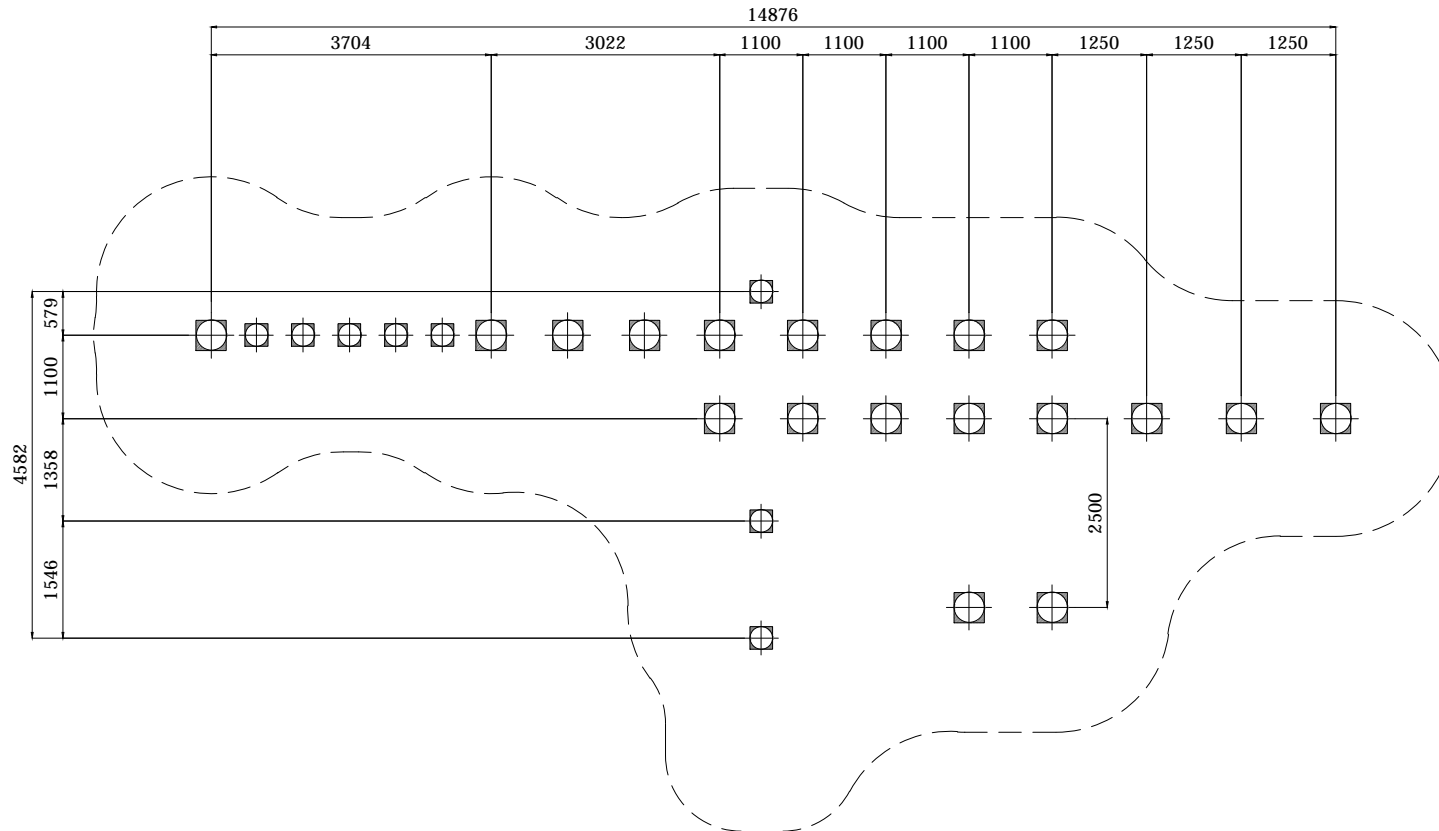
FOOTING LAYOUT
