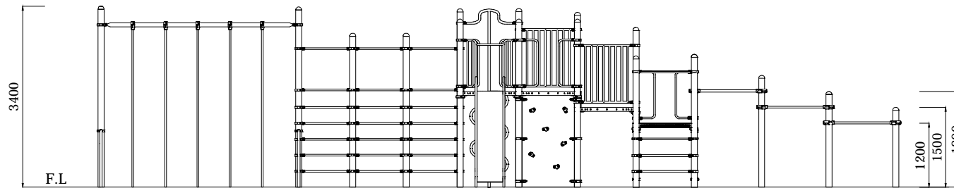
ELEVATION - FRONT
