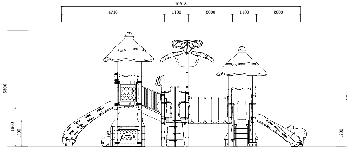
ELEVATION - FRONT
