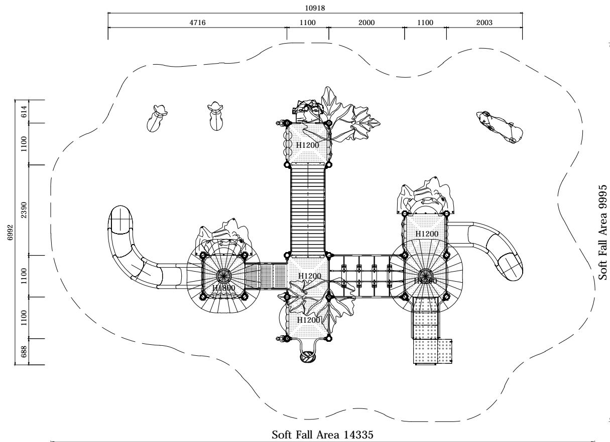
PLAN LAYOUT
