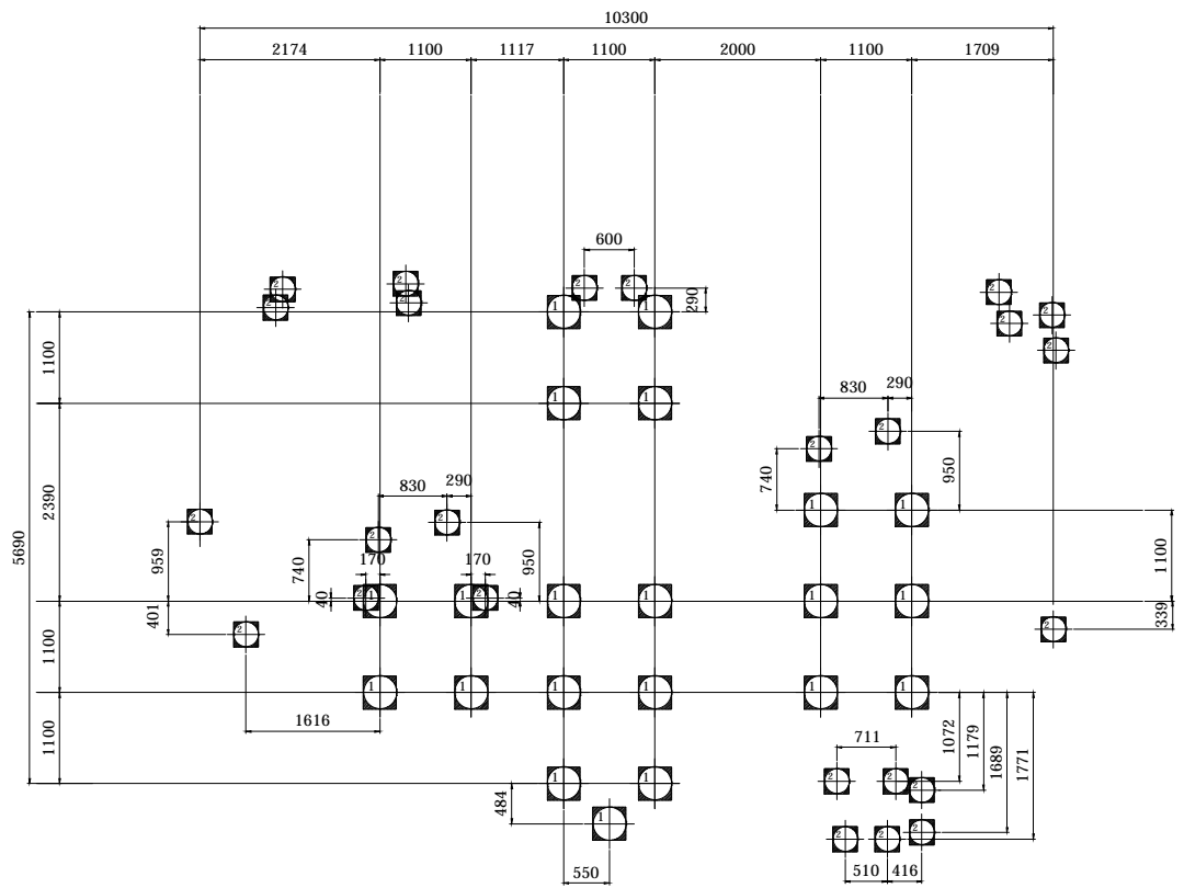
FOOTING LAYOUT
