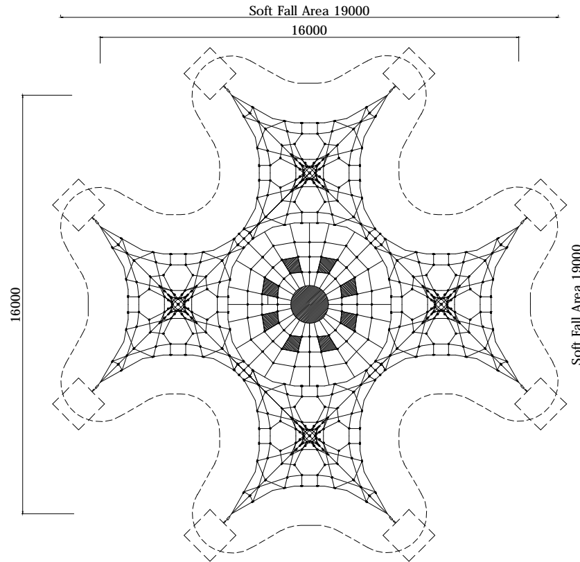
PLAN LAYOUT
