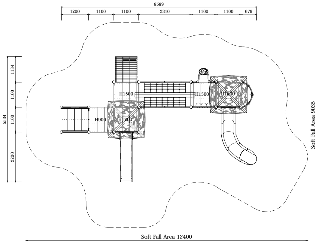
PLAN LAYOUT
