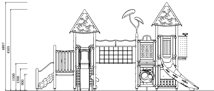
ELEVATION - FRONT
