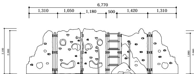
ELEVATION - FRONT
