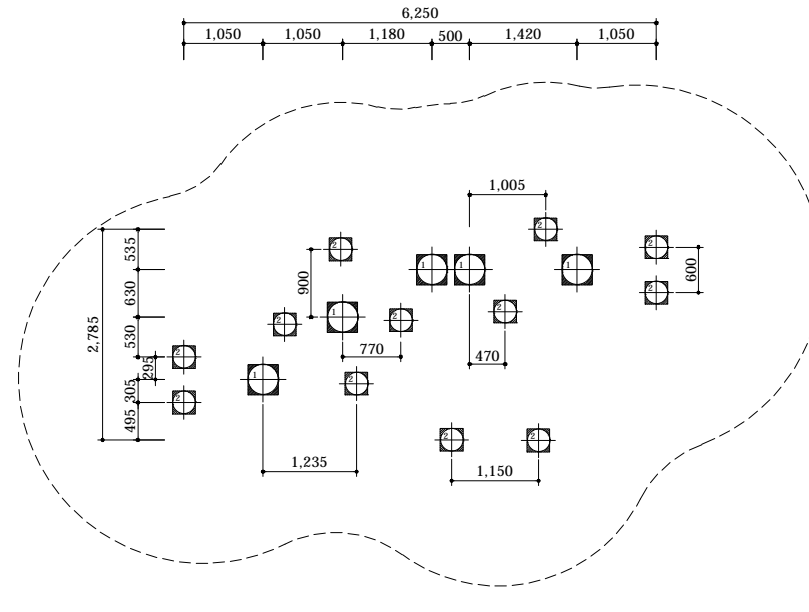
FOOTING LAYOUT
