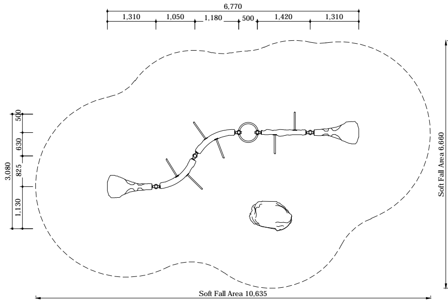
PLAN LAYOUT
