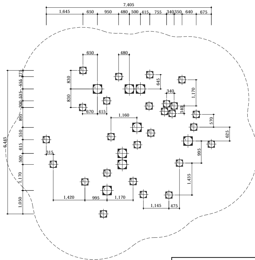
FOOTING LAYOUT
