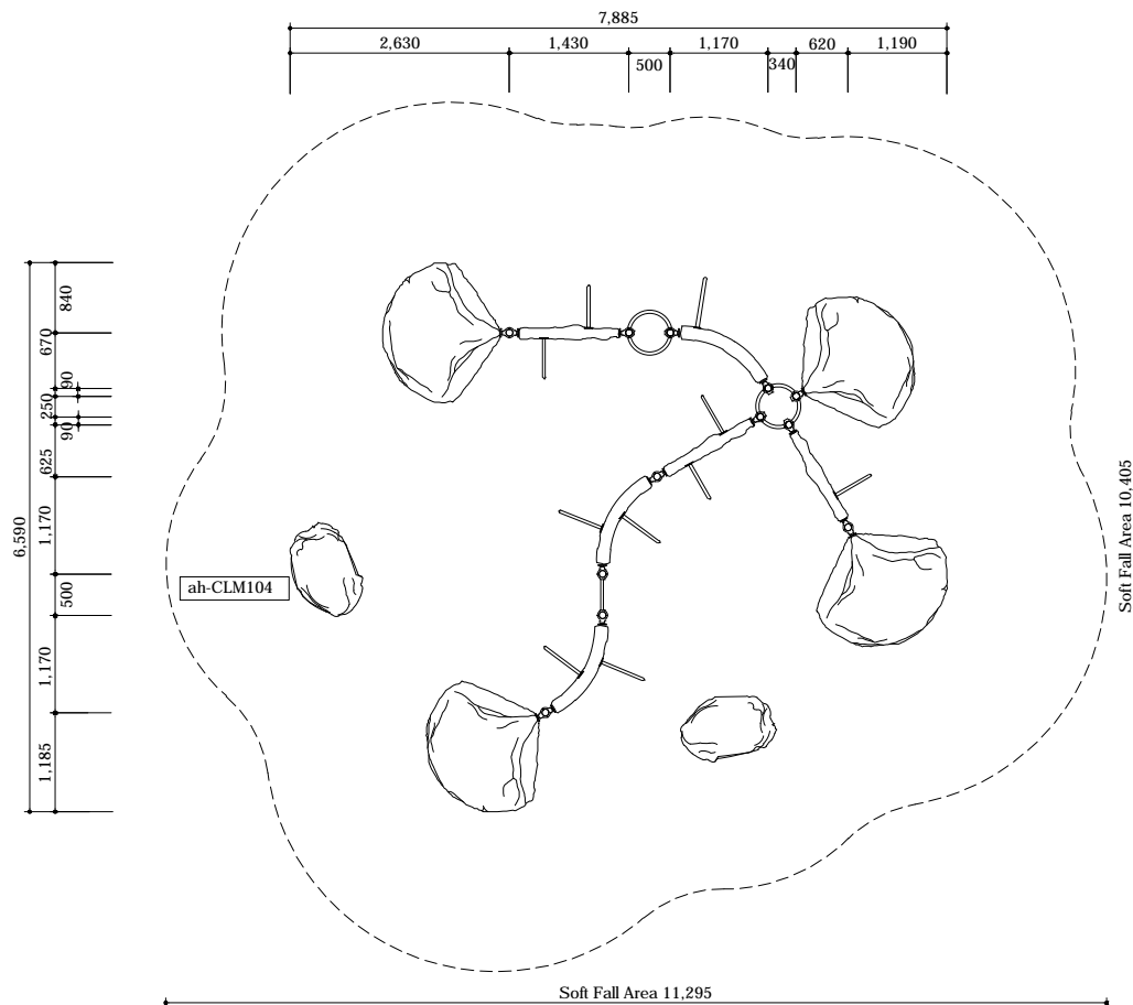
PLAN LAYOUT
