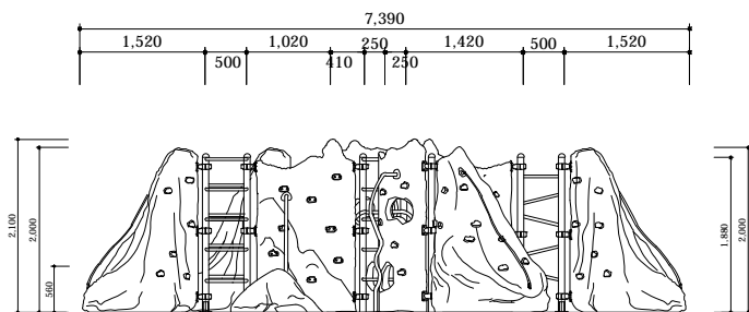
ELEVATION - FRONT
