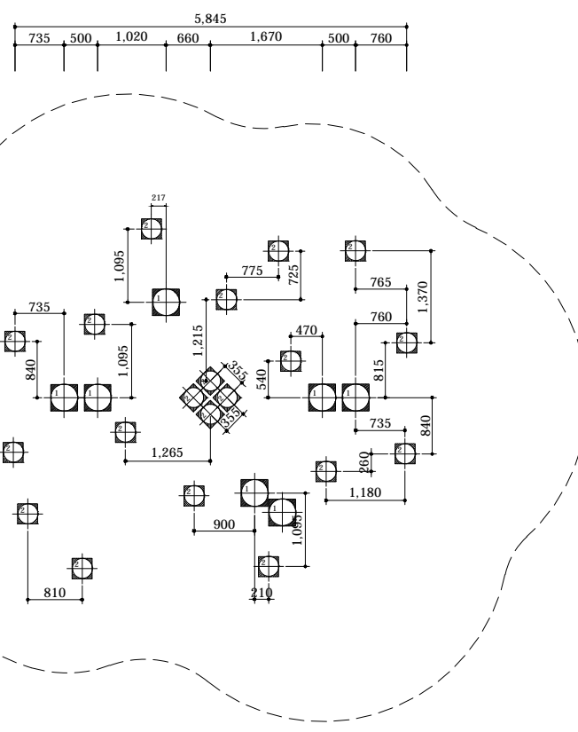
FOOTING LAYOUT
