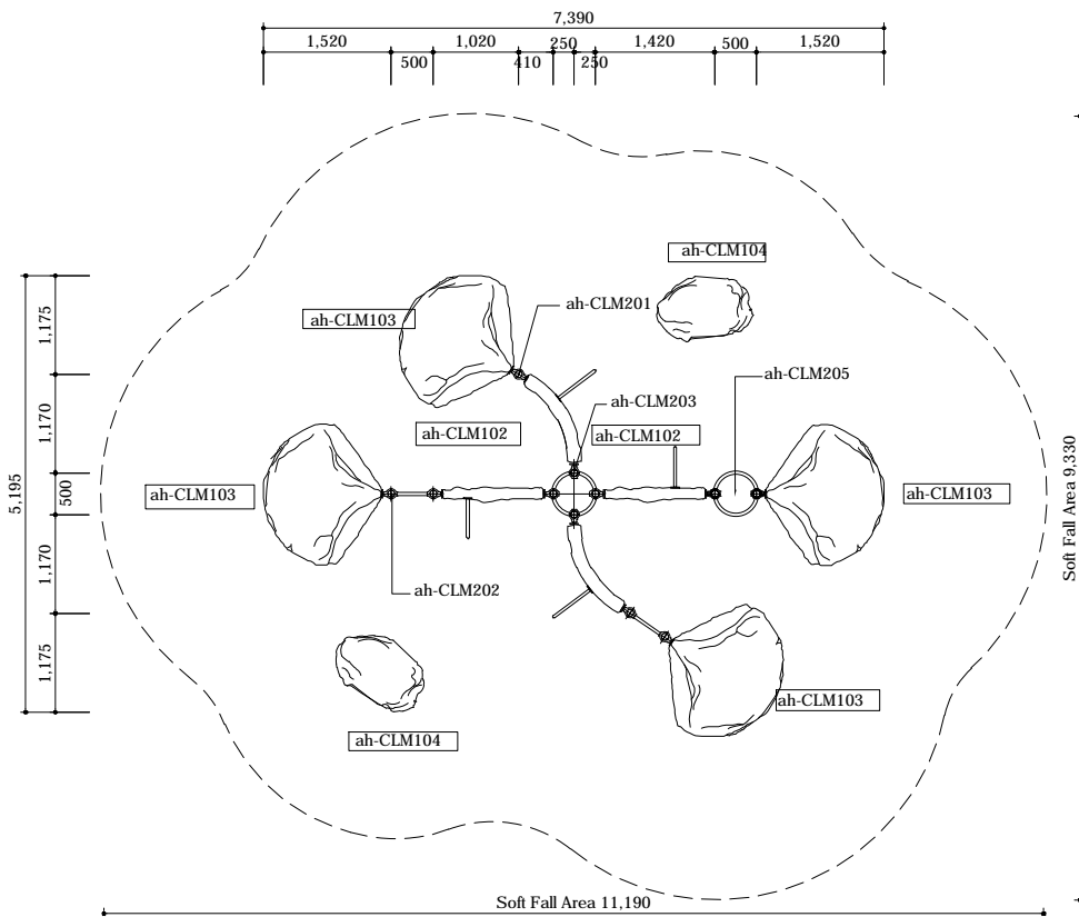
PLAN LAYOUT
