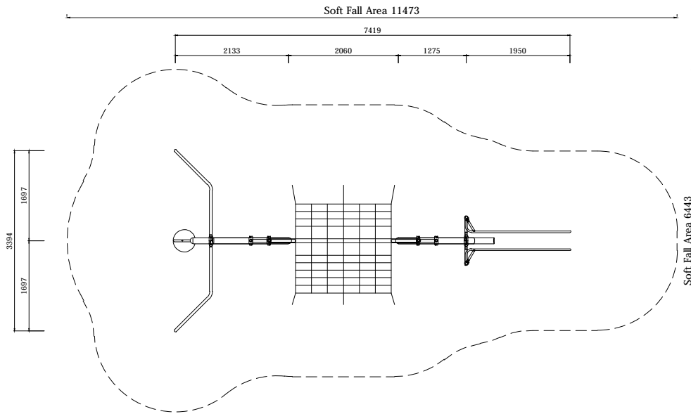
PLAN LAYOUT
