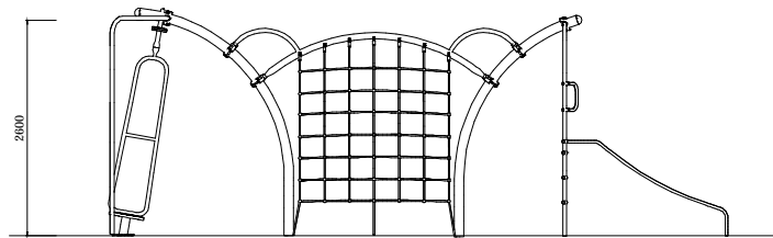
ELEVATION - FRONT
