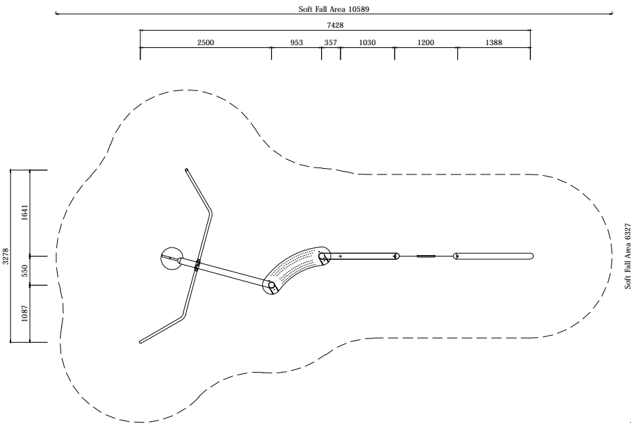
PLAN LAYOUT
