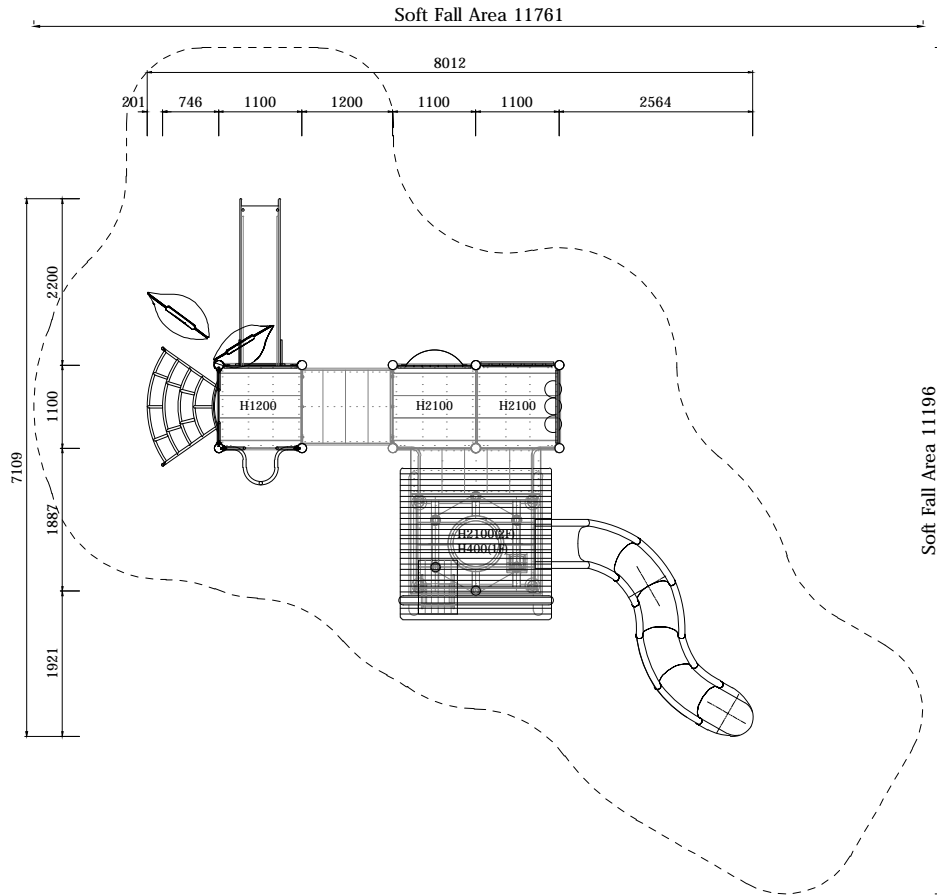
PLAN LAYOUT
