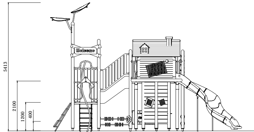
ELEVATION - FRONT
