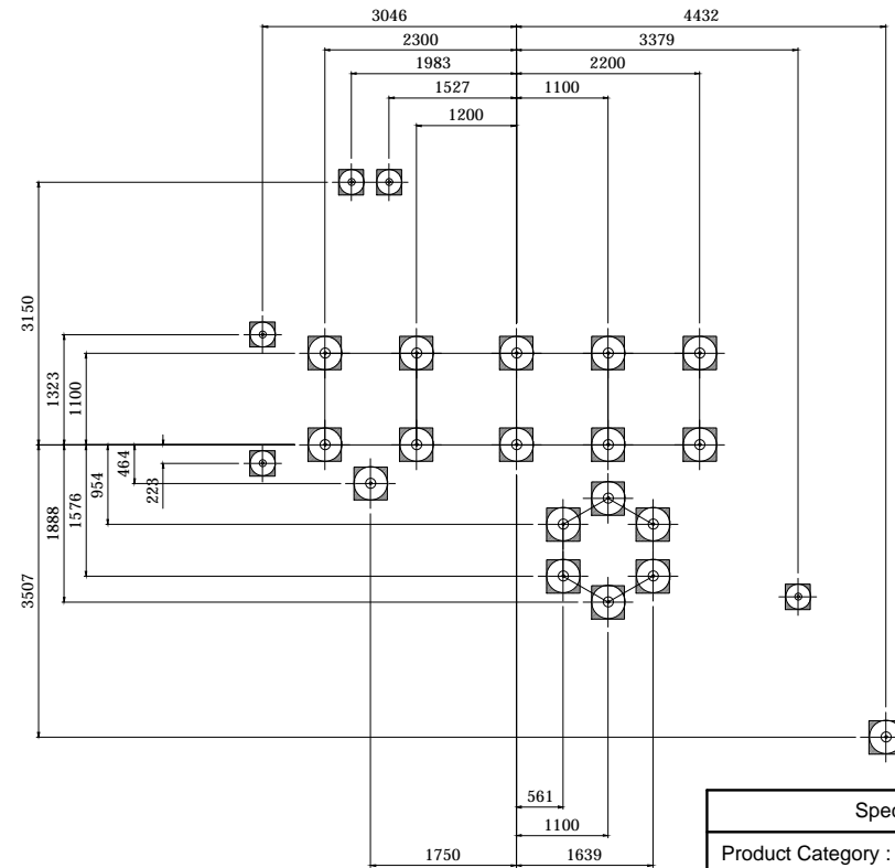
FOOTING LAYOUT
