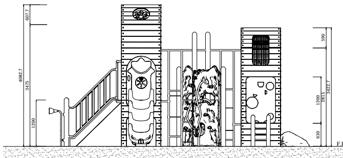
ELEVATION - FRONT
