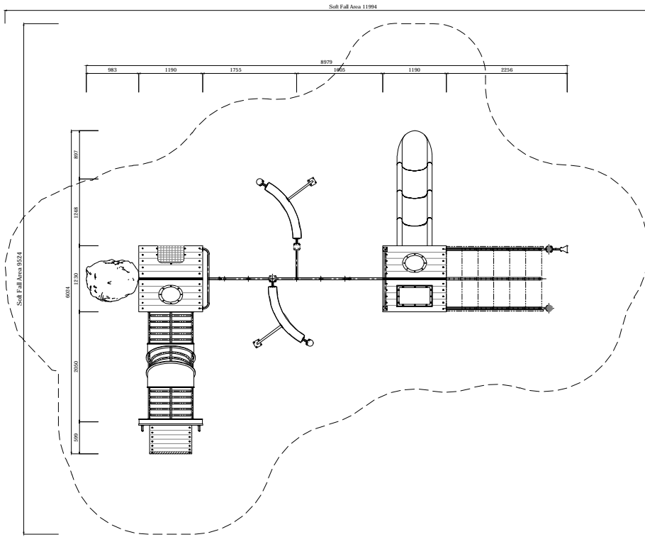
PLAN LAYOUT
