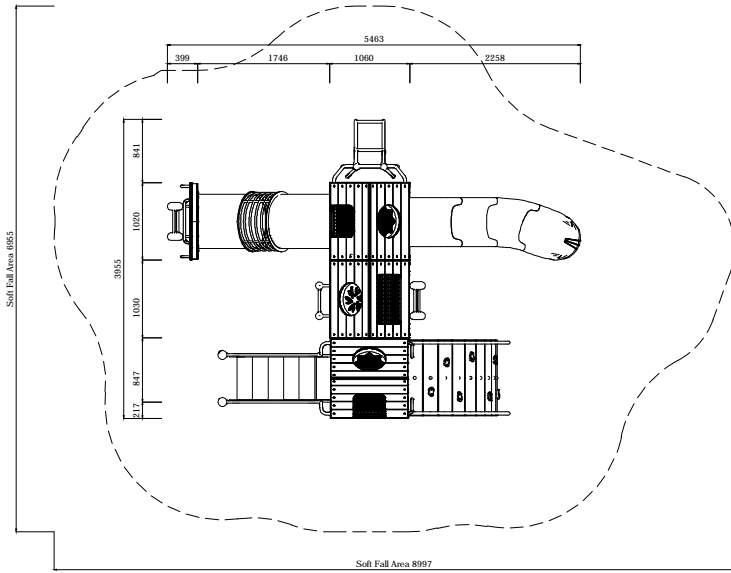
PLAN LAYOUT
