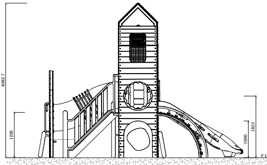
ELEVATION - FRONT
