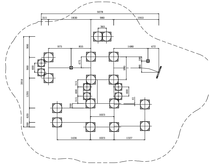
FOOTING LAYOUT
