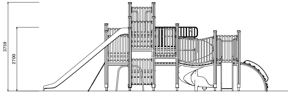
ELEVATION - FRONT
