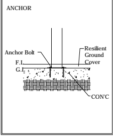
TYPICAL FOOTING DETAILS
