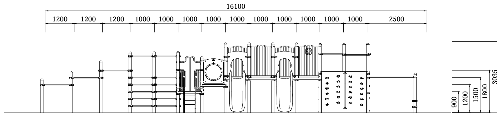
ELEVATION - FRONT
