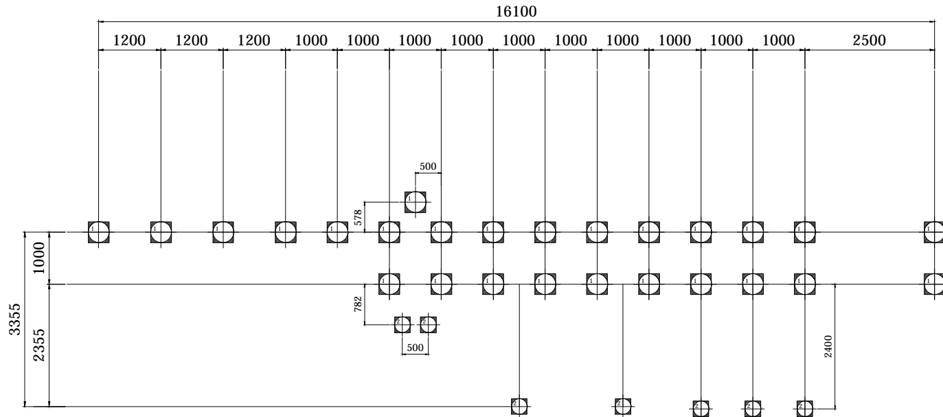
FOOTING LAYOUT
