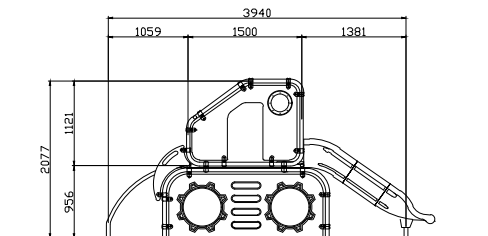
ELEVATION - FRONT
