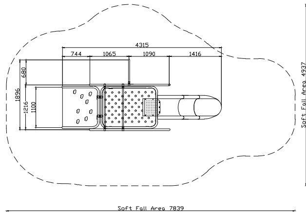
PLAN LAYOUT
